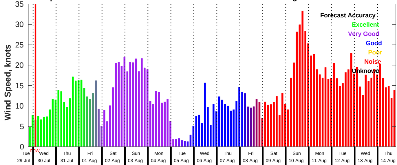
GFS Wind Speed Forecast for NDBC 41004 from 29-Jul-2025 19:00:00 to 14-Aug-2025 19:00:00
