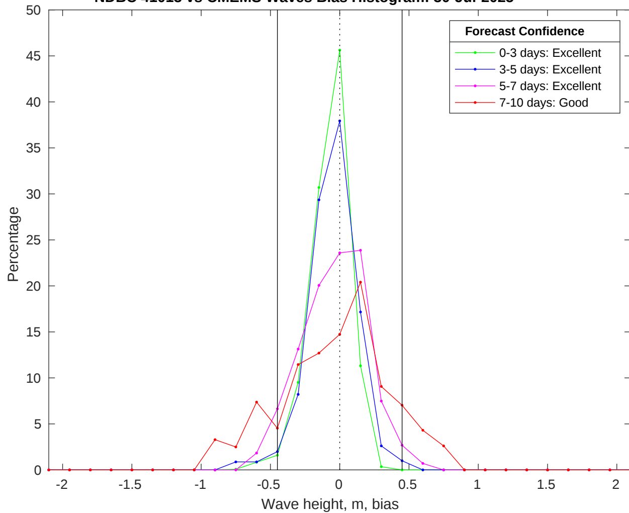
NDBC 41013 vs CMEMS Waves Bias Histogram: 30-Jul-2025
