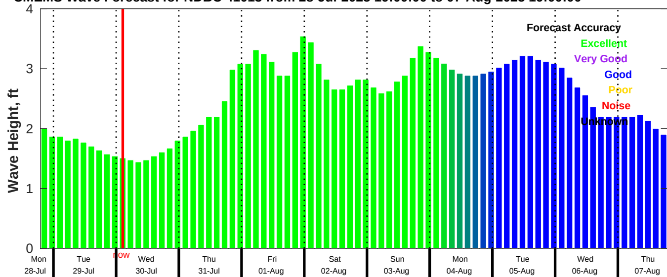
CMEMS Wave Forecast for NDBC 41013 from 28-Jul-2025 19:00:00 to 07-Aug-2025 19:00:00
