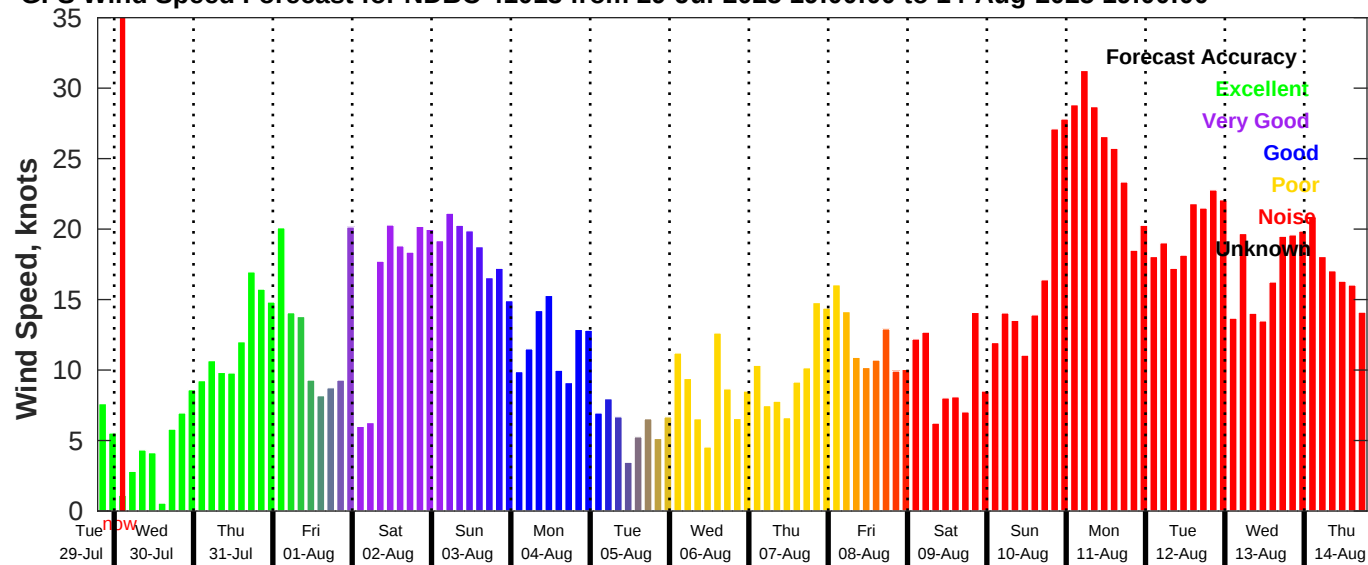
GFS Wind Speed Forecast for NDBC 41013 from 29-Jul-2025 19:00:00 to 14-Aug-2025 19:00:00
