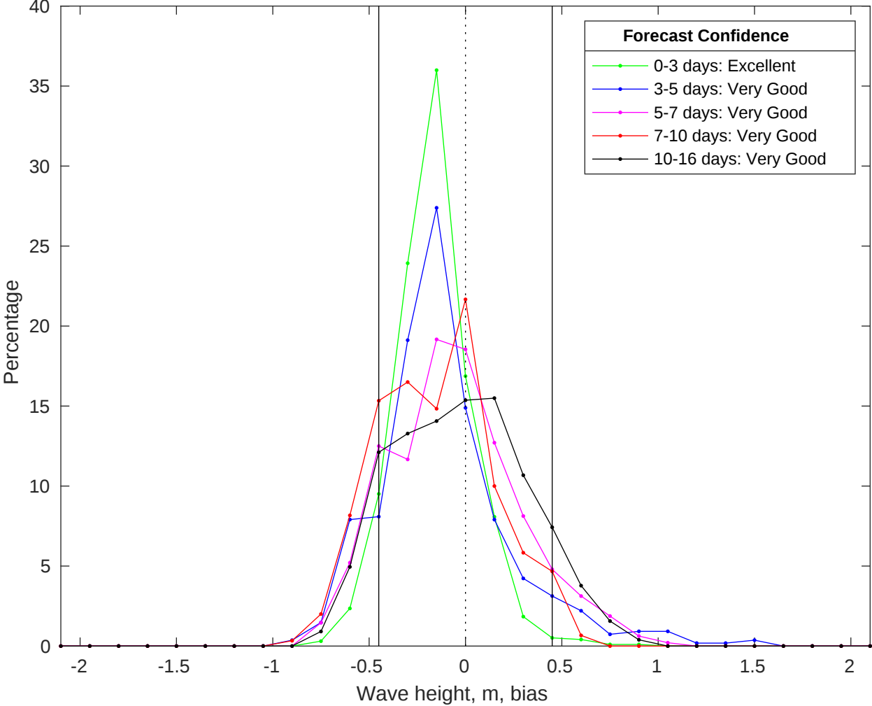
NDBC 41040 vs GFS Waves Bias Histogram: 30-Jul-2025
