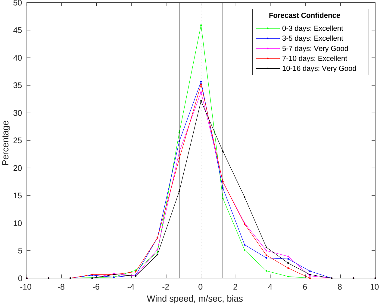
NDBC 41040 vs GFS Winds Bias Histogram: 30-Jul-2025
