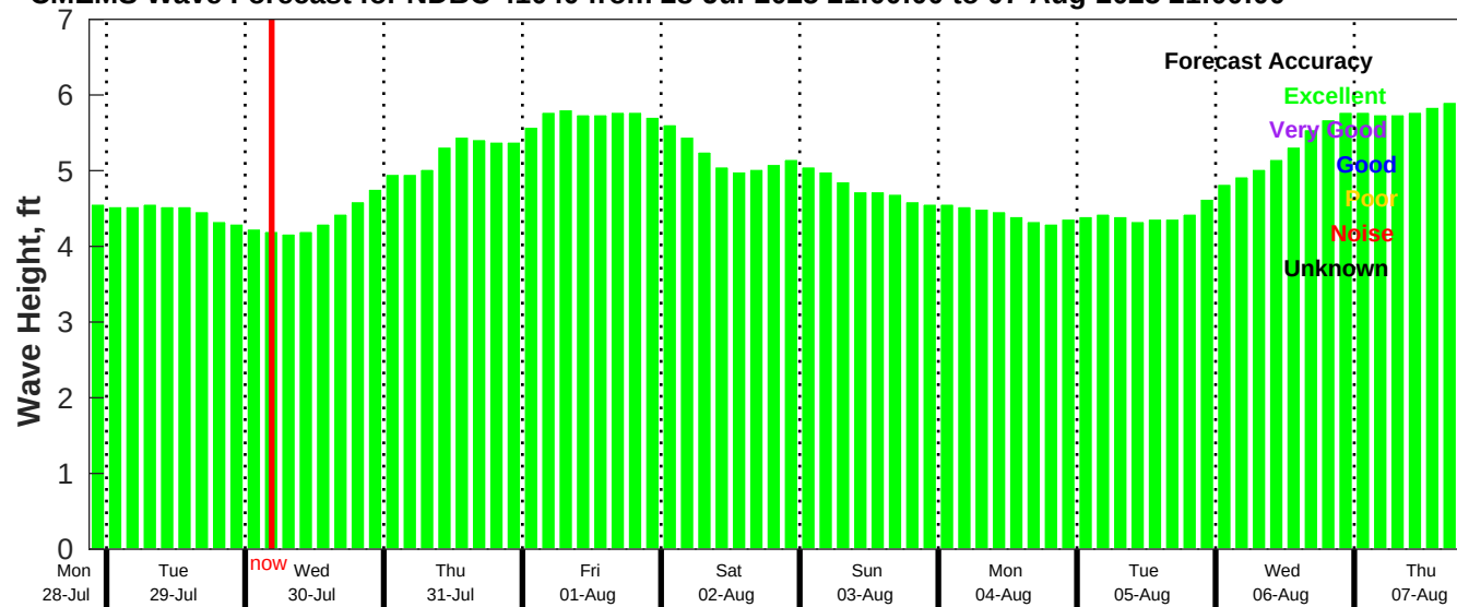
CMEMS Wave Forecast for NDBC 41040 from 28-Jul-2025 21:00:00 to 07-Aug-2025 21:00:00
