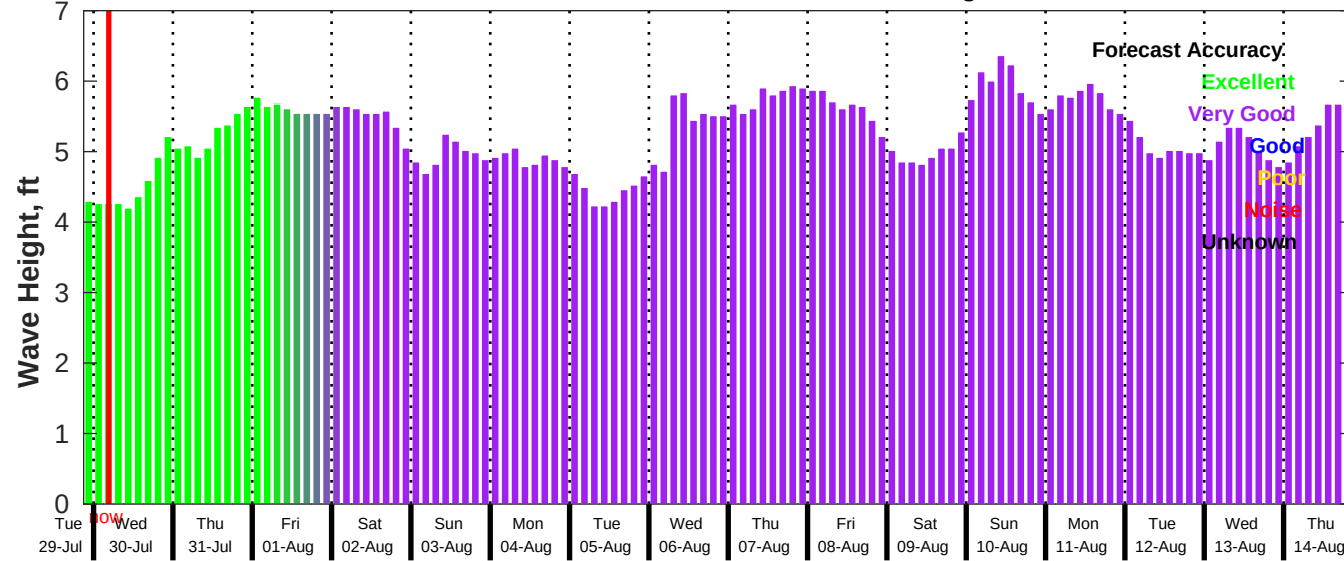
GFS Wave Forecast for NDBC 41040 from 29-Jul-2025 21:00:00 to 14-Aug-2025 21:00:00
