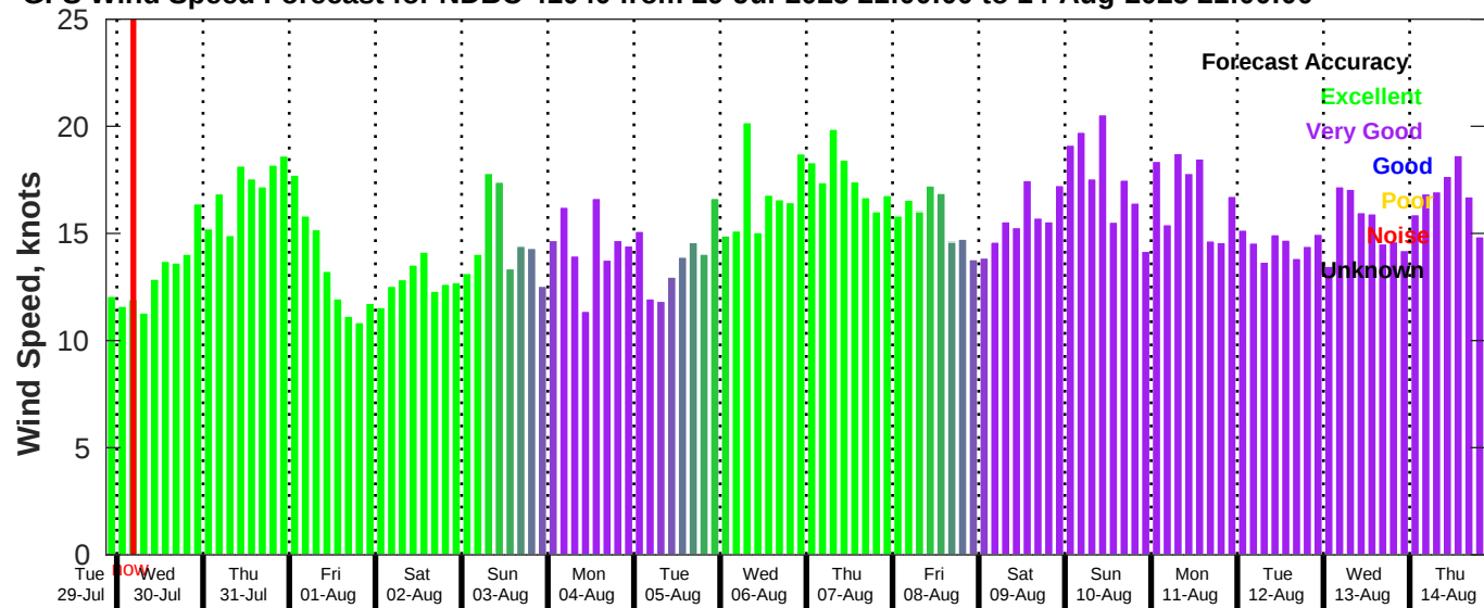
GFS Wind Speed Forecast for NDBC 41040 from 29-Jul-2025 21:00:00 to 14-Aug-2025 21:00:00
