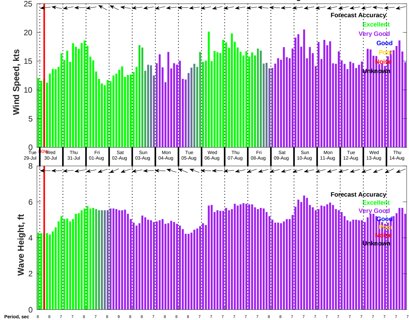
Wind & Wave Forecast for NDBC 41040 from 29-Jul-2025 21:00:00 to 14-Aug-2025 21:00:00
