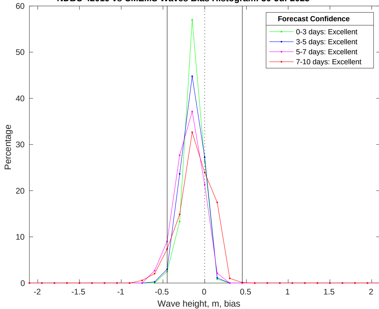
NDBC 42019 vs CMEMS Waves Bias Histogram: 30-Jul-2025
