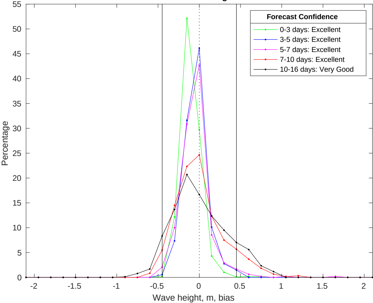
NDBC 42019 vs GFS Waves Bias Histogram: 30-Jul-2025
