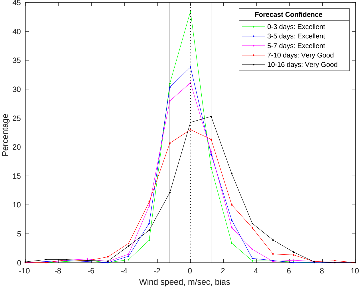
NDBC 42019 vs GFS Winds Bias Histogram: 30-Jul-2025
