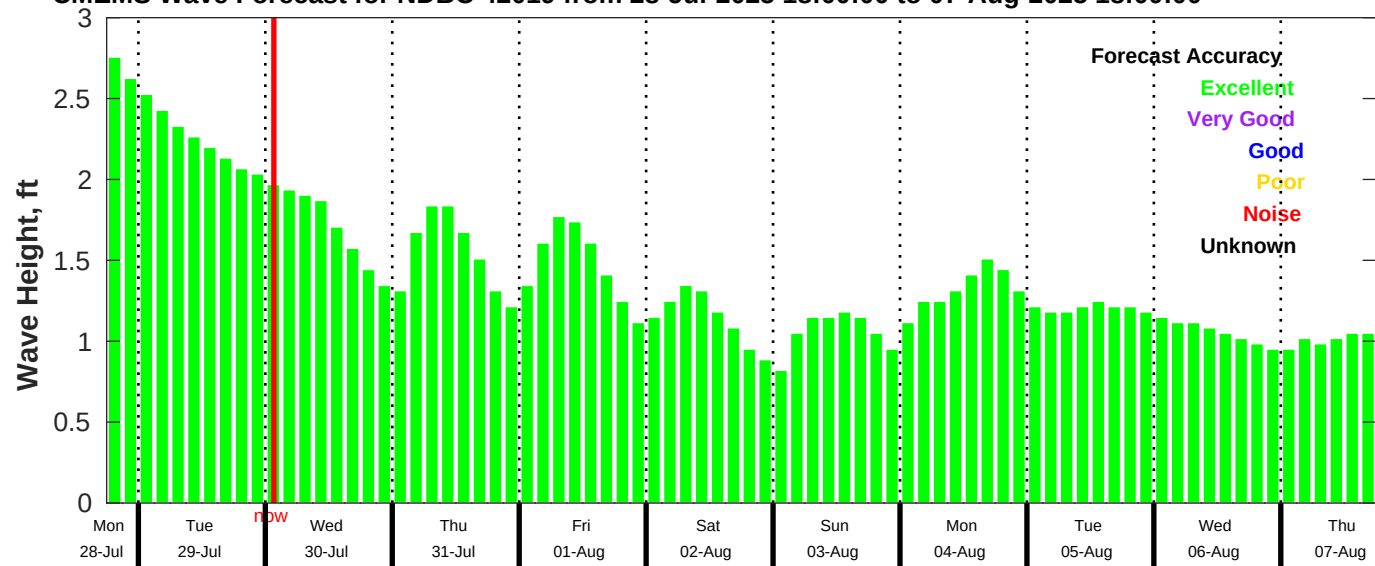
CMEMS Wave Forecast for NDBC 42019 from 28-Jul-2025 18:00:00 to 07-Aug-2025 18:00:00
