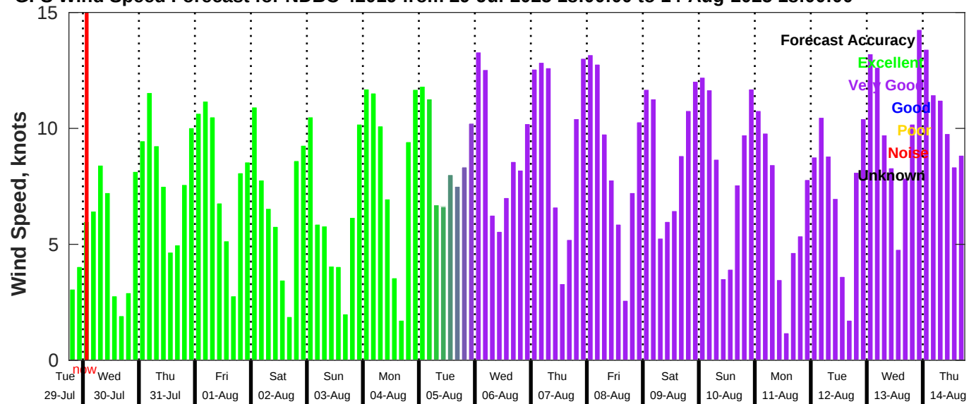
GFS Wind Speed Forecast for NDBC 42019 from 29-Jul-2025 18:00:00 to 14-Aug-2025 18:00:00
