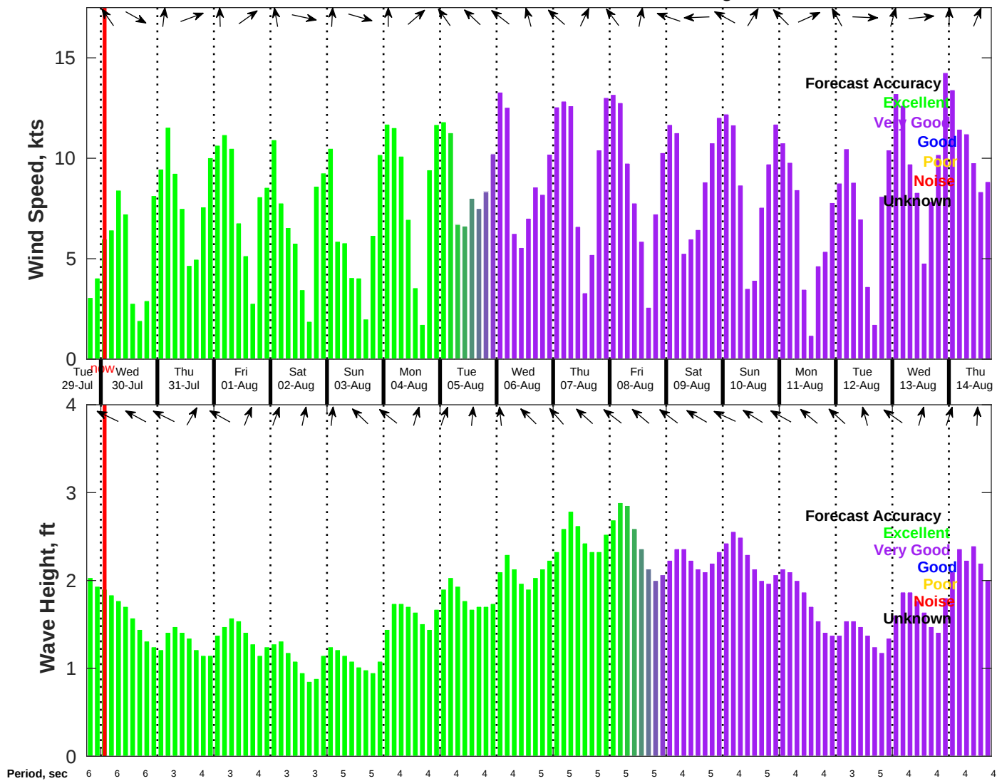
Wind & Wave Forecast for NDBC 42019 from 29-Jul-2025 18:00:00 to 14-Aug-2025 18:00:00
