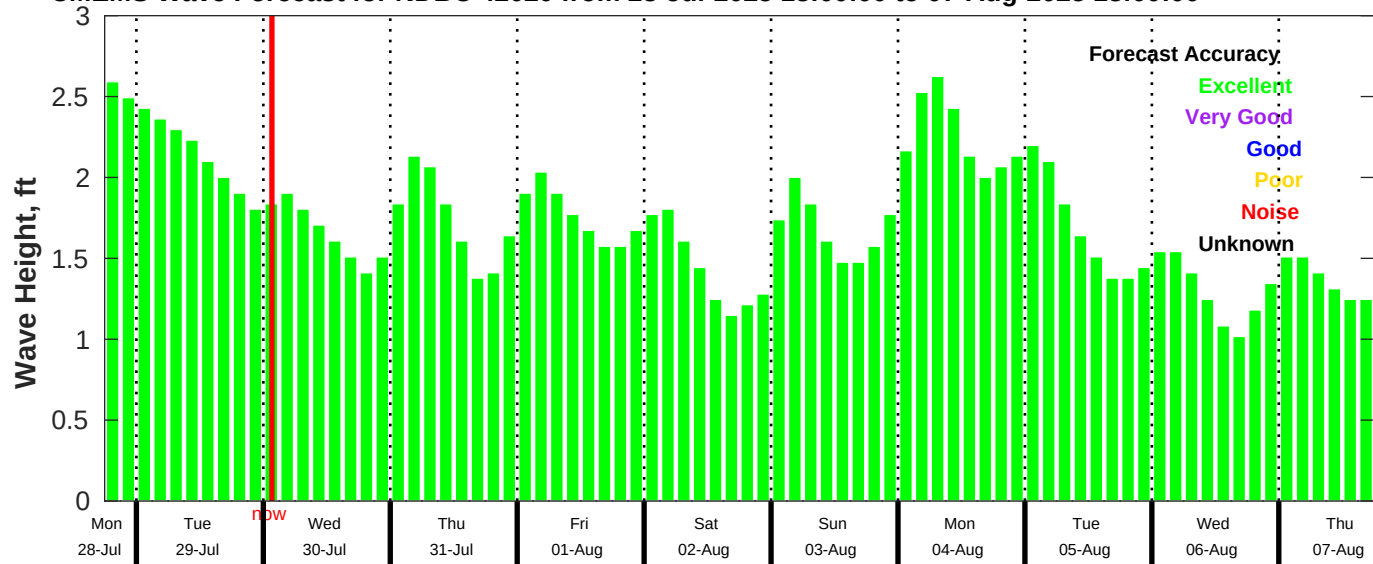
CMEMS Wave Forecast for NDBC 42020 from 28-Jul-2025 18:00:00 to 07-Aug-2025 18:00:00
