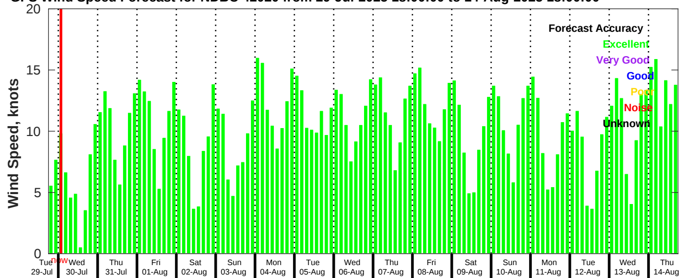
GFS Wind Speed Forecast for NDBC 42020 from 29-Jul-2025 18:00:00 to 14-Aug-2025 18:00:00
