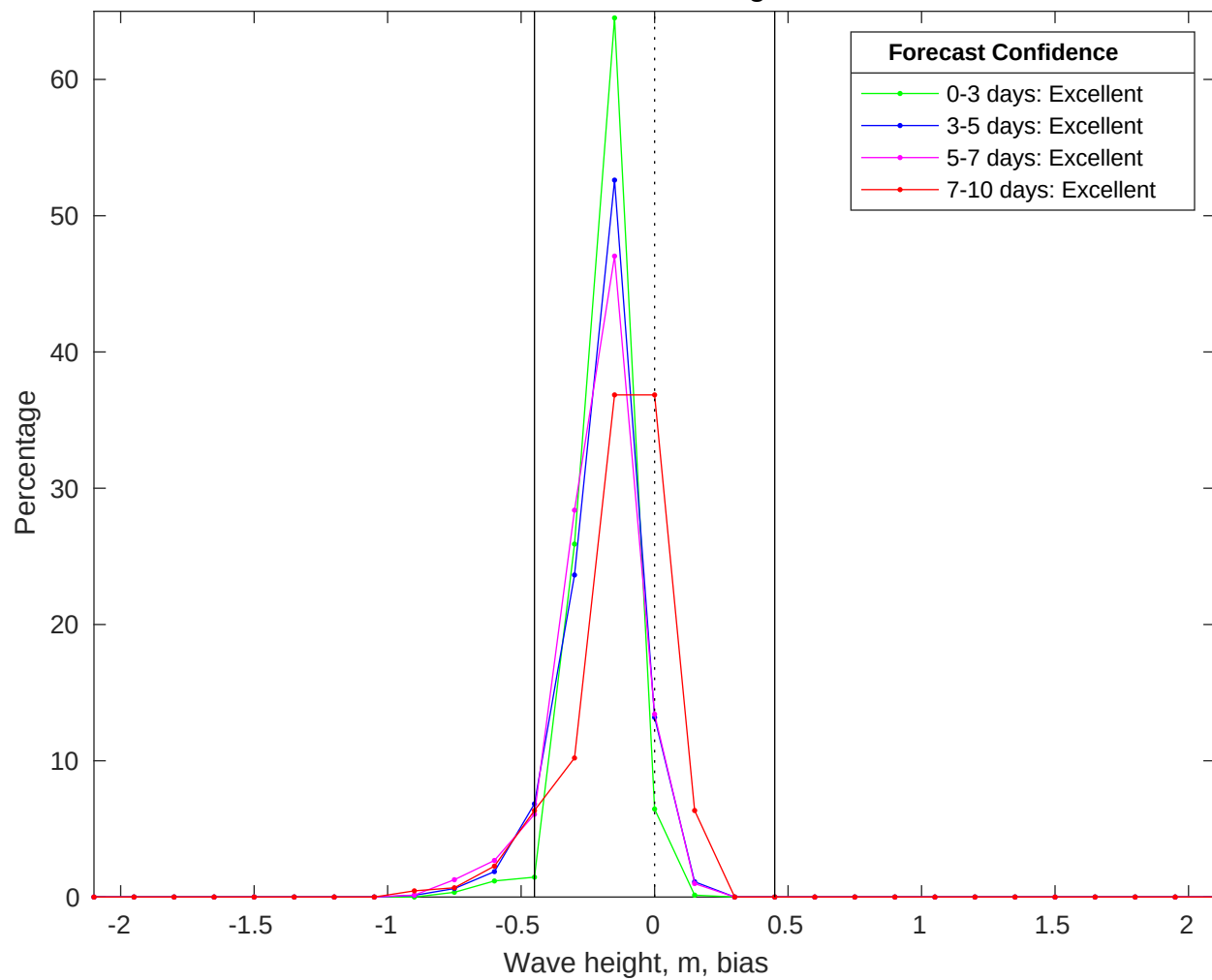
NDBC 42035 vs CMEMS Waves Bias Histogram: 30-Jul-2025
