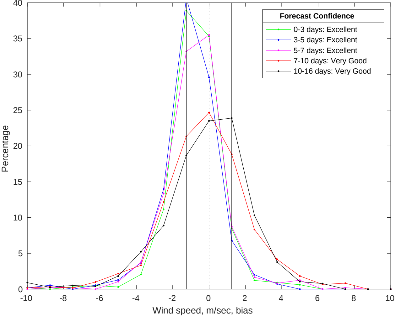
NDBC 42035 vs GFS Winds Bias Histogram: 30-Jul-2025
