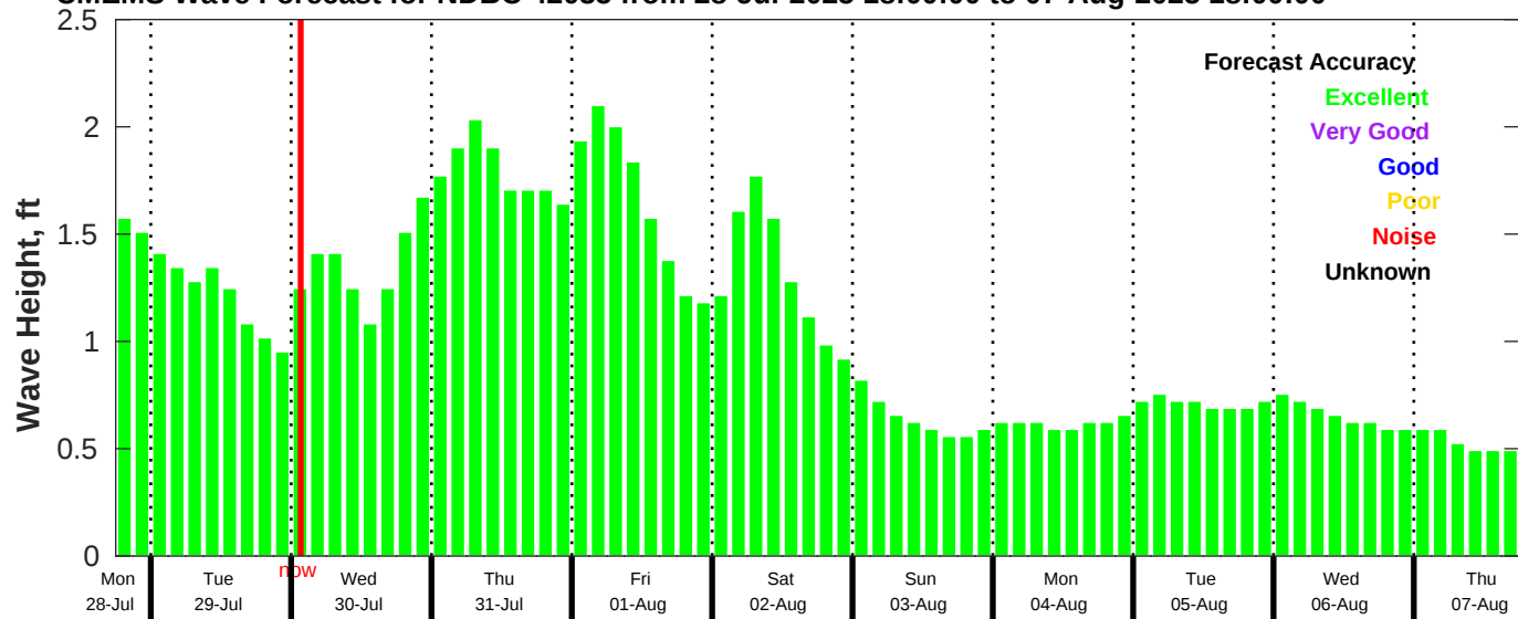
CMEMS Wave Forecast for NDBC 42035 from 28-Jul-2025 18:00:00 to 07-Aug-2025 18:00:00
