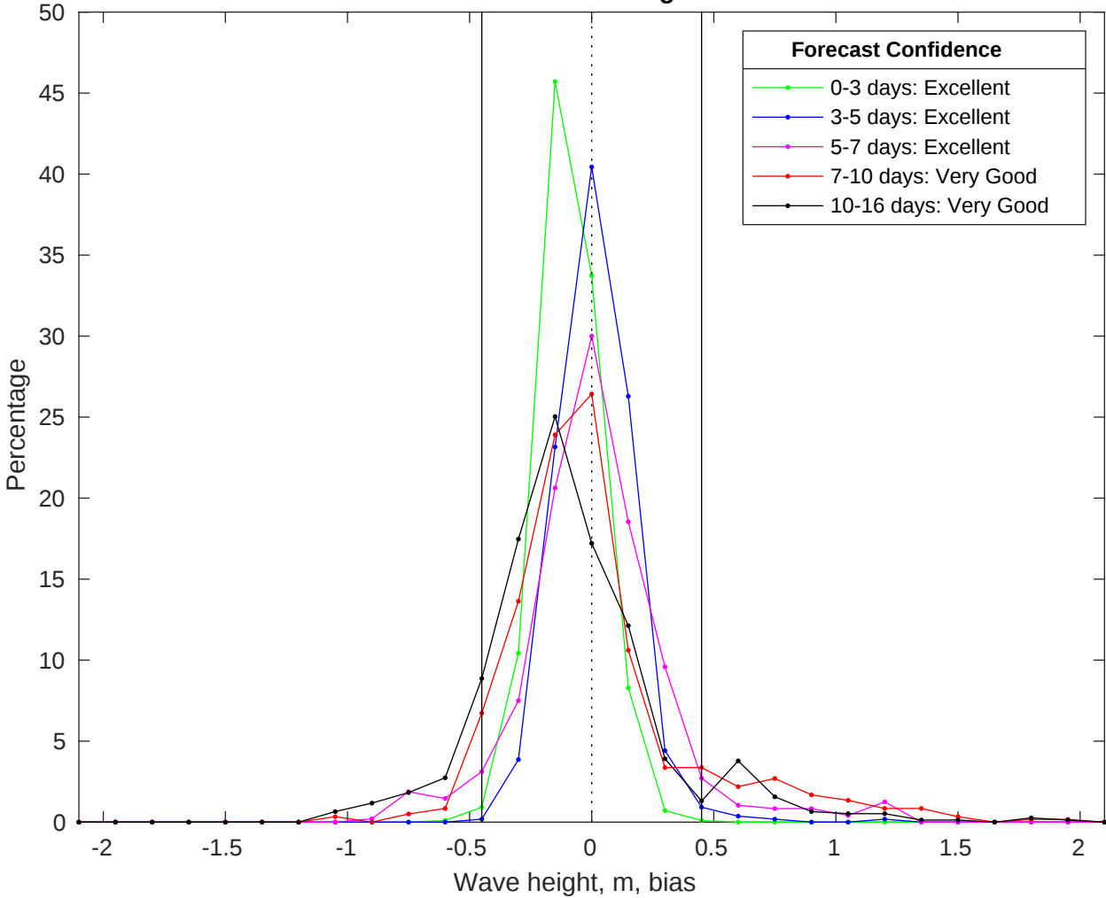
NDBC 42036 vs GFS Waves Bias Histogram: 30-Jul-2025
