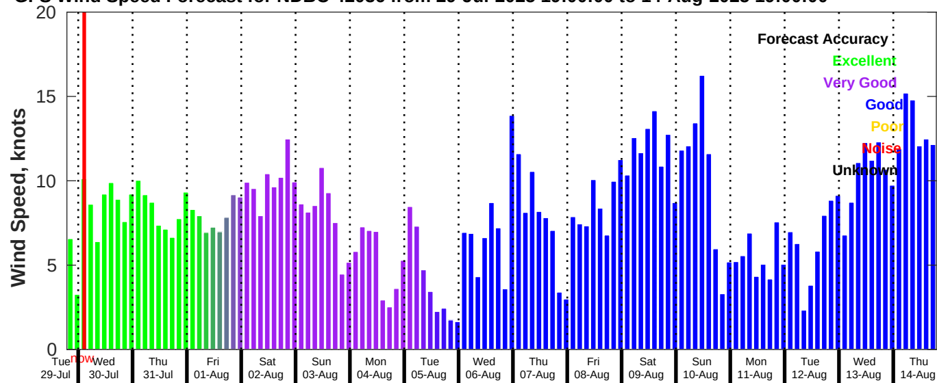
GFS Wind Speed Forecast for NDBC 42036 from 29-Jul-2025 19:00:00 to 14-Aug-2025 19:00:00
