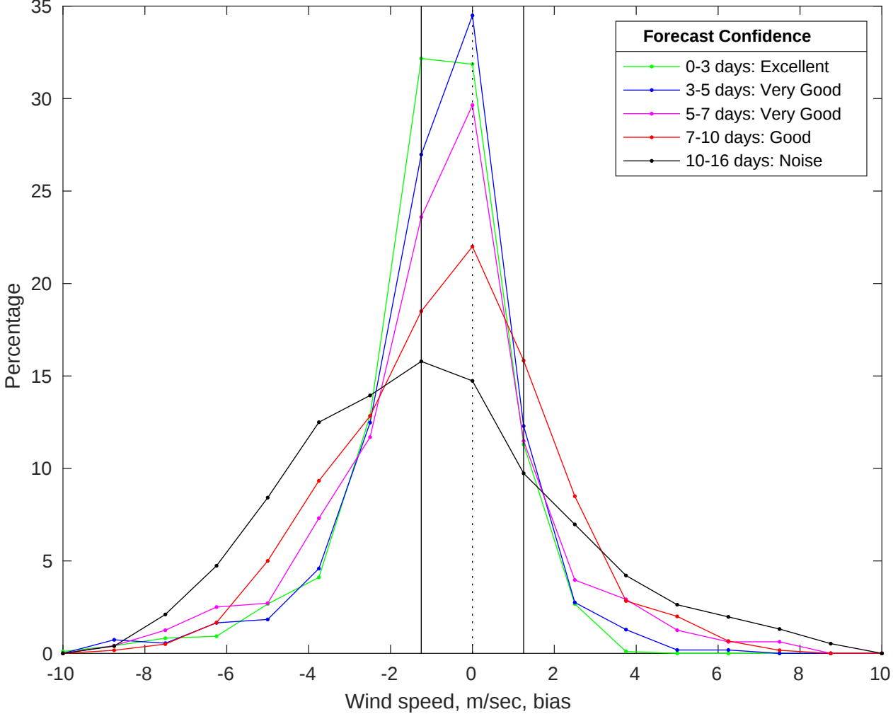
NDBC 42040 vs GFS Winds Bias Histogram: 30-Jul-2025
