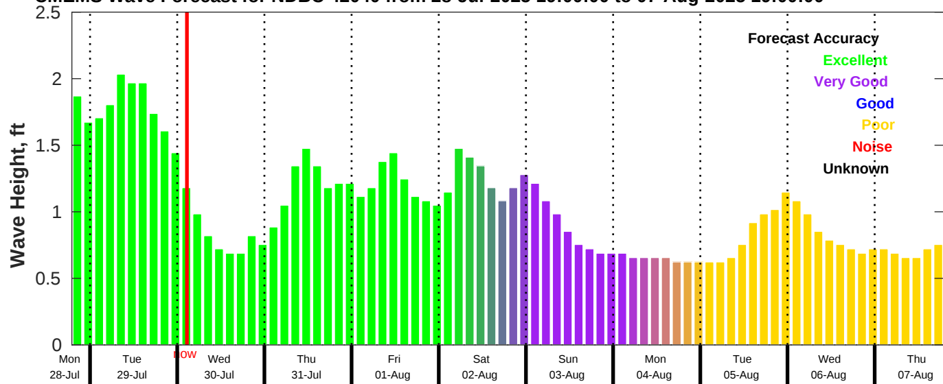
CMEMS Wave Forecast for NDBC 42040 from 28-Jul-2025 19:00:00 to 07-Aug-2025 19:00:00
