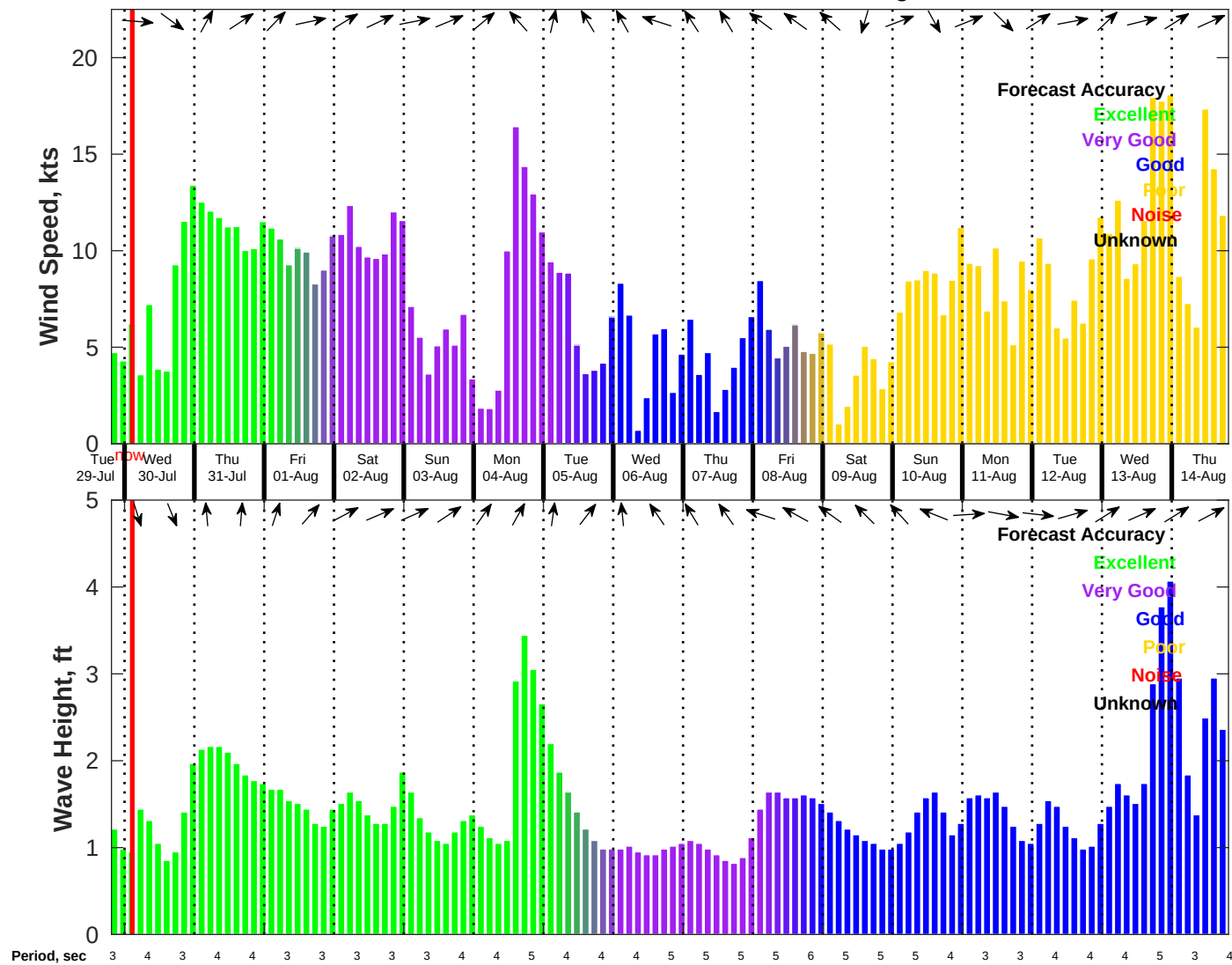
Wind & Wave Forecast for NDBC 42040 from 29-Jul-2025 19:00:00 to 14-Aug-2025 19:00:00
