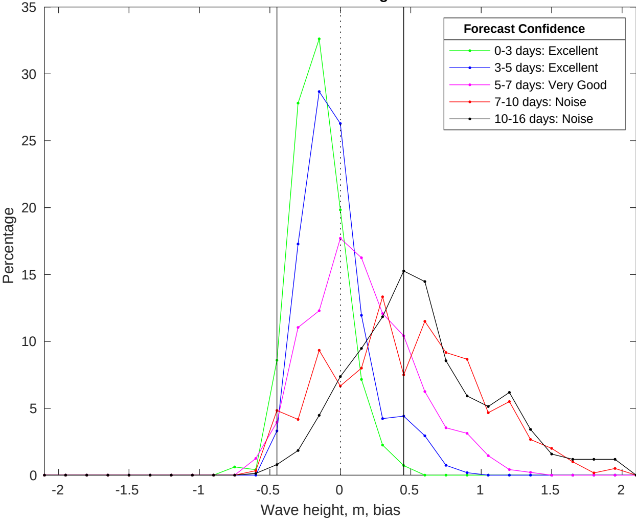
NDBC 46011 vs GFS Waves Bias Histogram: 30-Jul-2025
