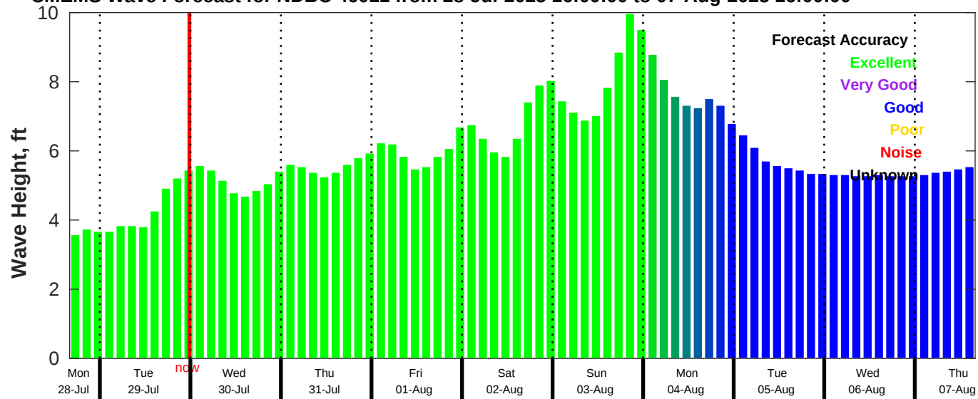
CMEMS Wave Forecast for NDBC 46011 from 28-Jul-2025 16:00:00 to 07-Aug-2025 16:00:00
