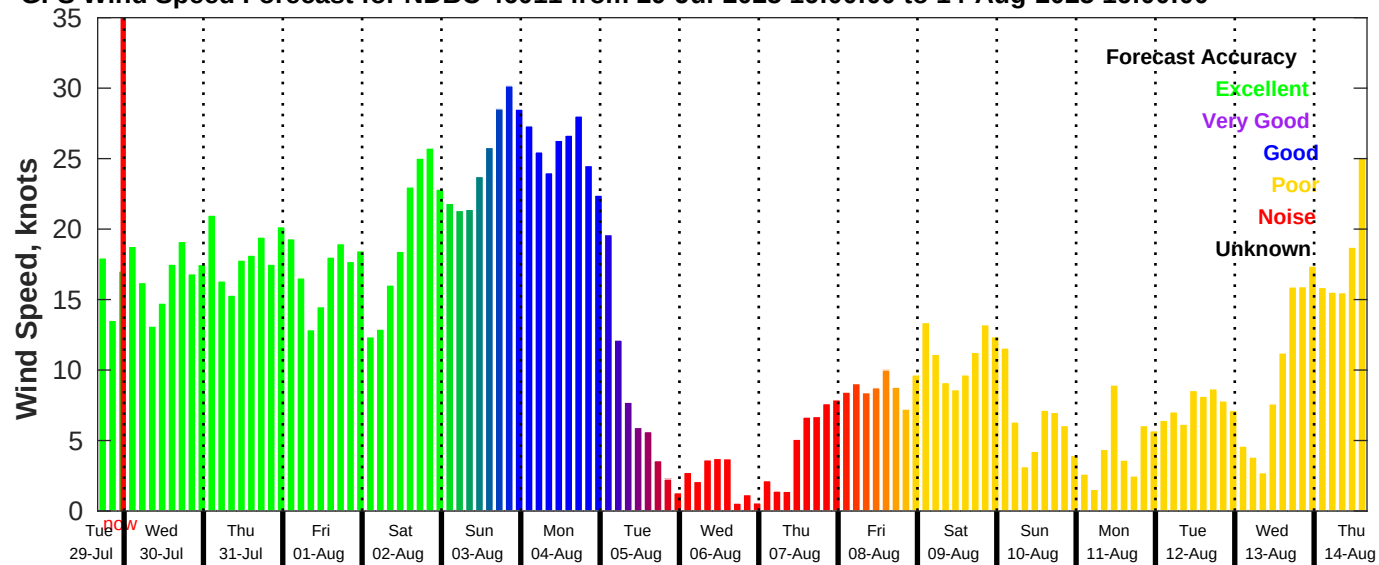
GFS Wind Speed Forecast for NDBC 46011 from 29-Jul-2025 16:00:00 to 14-Aug-2025 16:00:00
