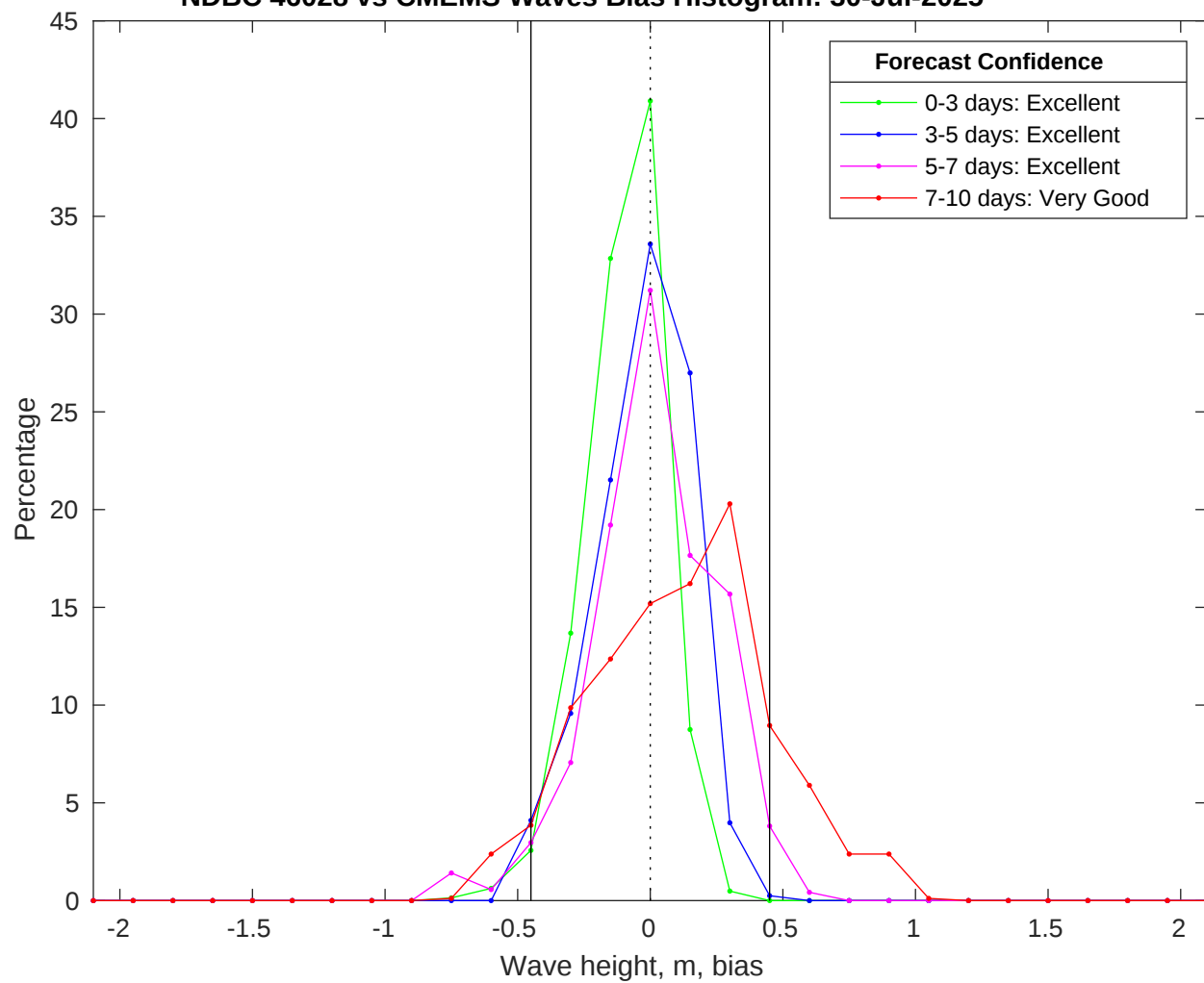
NDBC 46028 vs CMEMS Waves Bias Histogram: 30-Jul-2025
