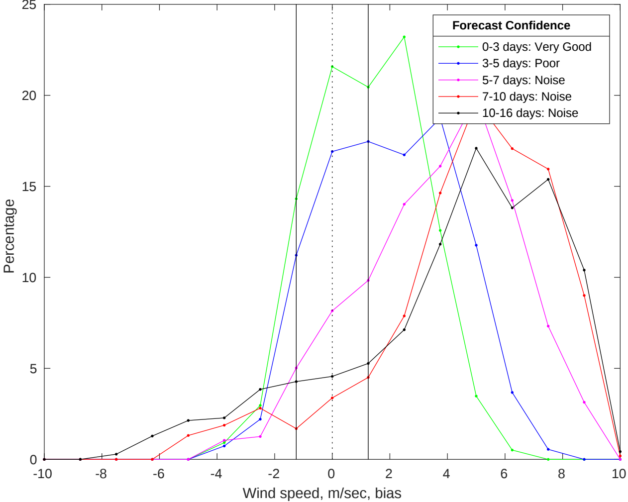
NDBC 46028 vs GFS Winds Bias Histogram: 30-Jul-2025
