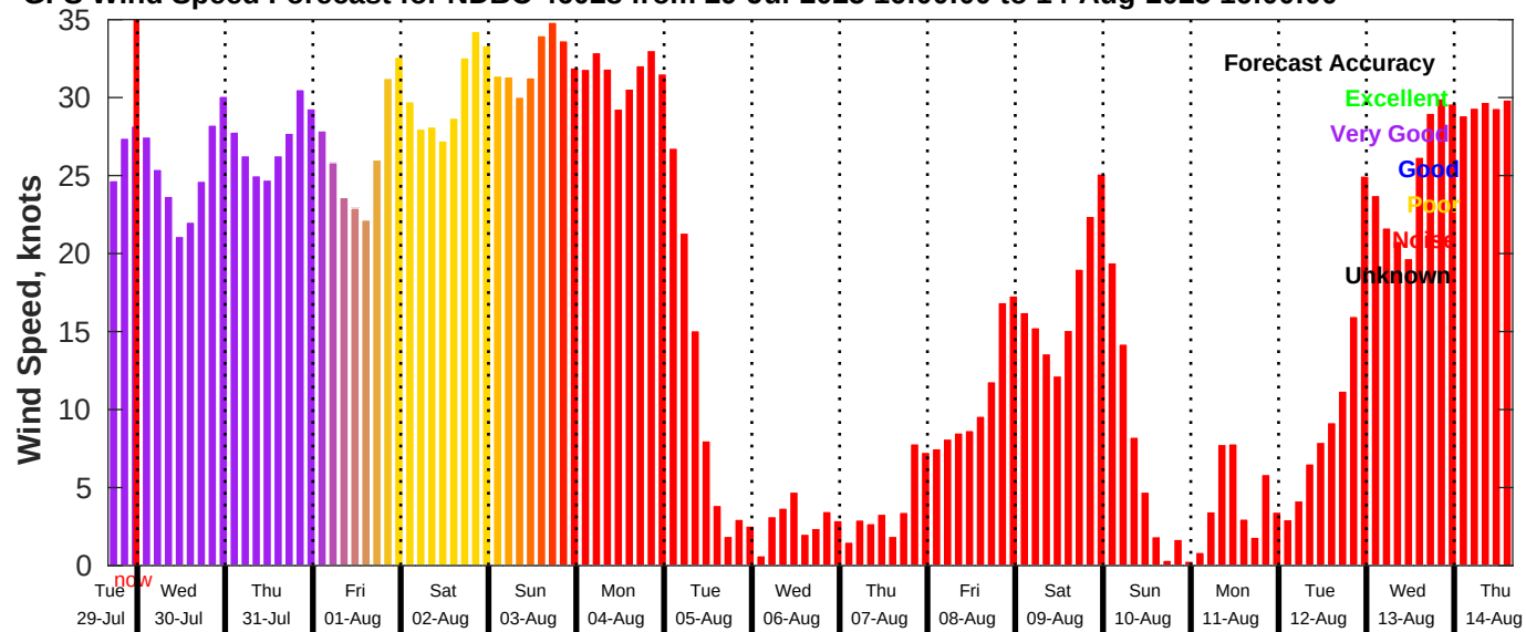
GFS Wind Speed Forecast for NDBC 46028 from 29-Jul-2025 16:00:00 to 14-Aug-2025 16:00:00
