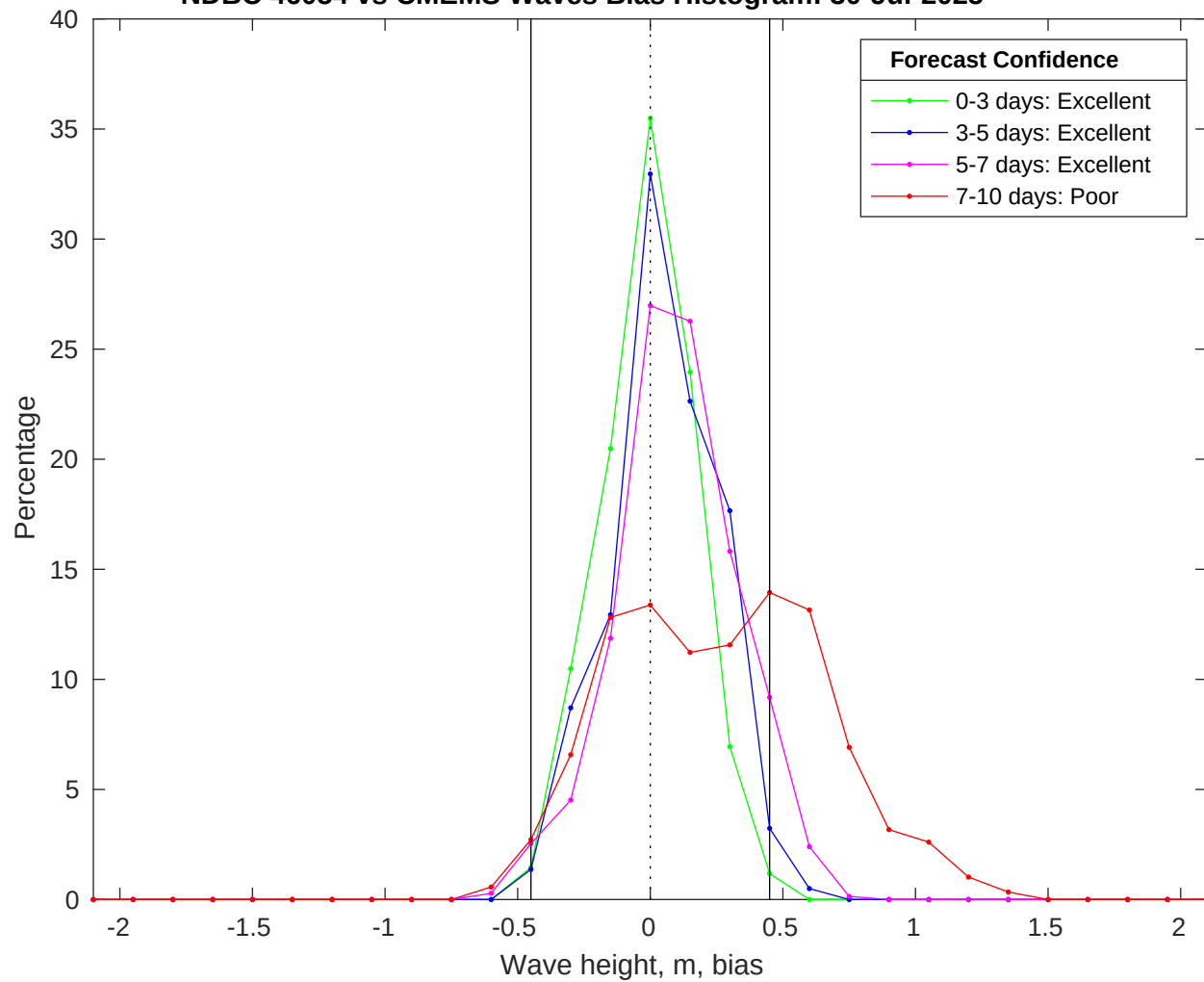
NDBC 46054 vs CMEMS Waves Bias Histogram: 30-Jul-2025
