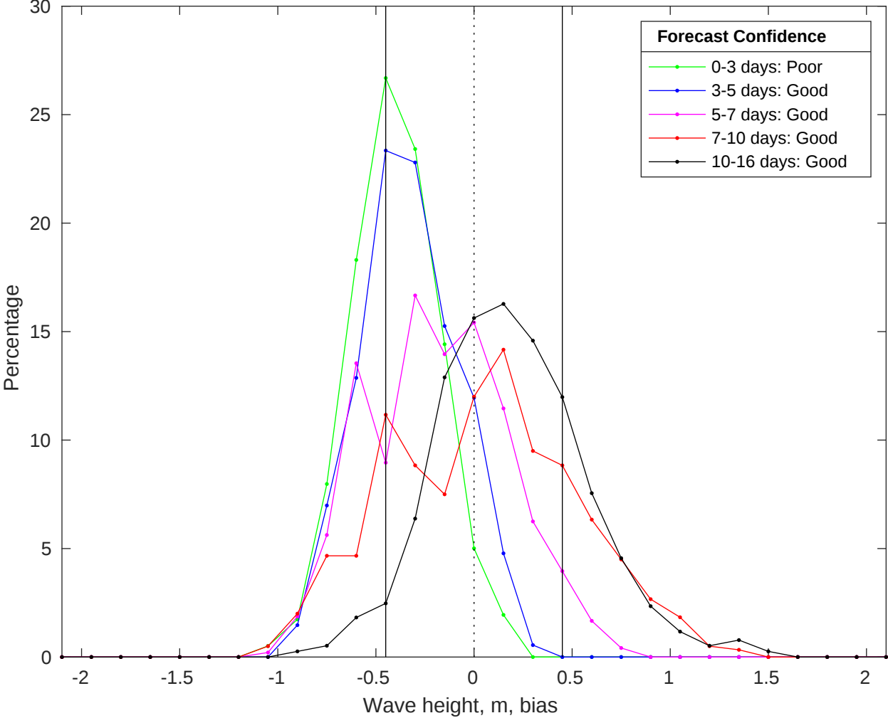
NDBC 46054 vs GFS Waves Bias Histogram: 30-Jul-2025
