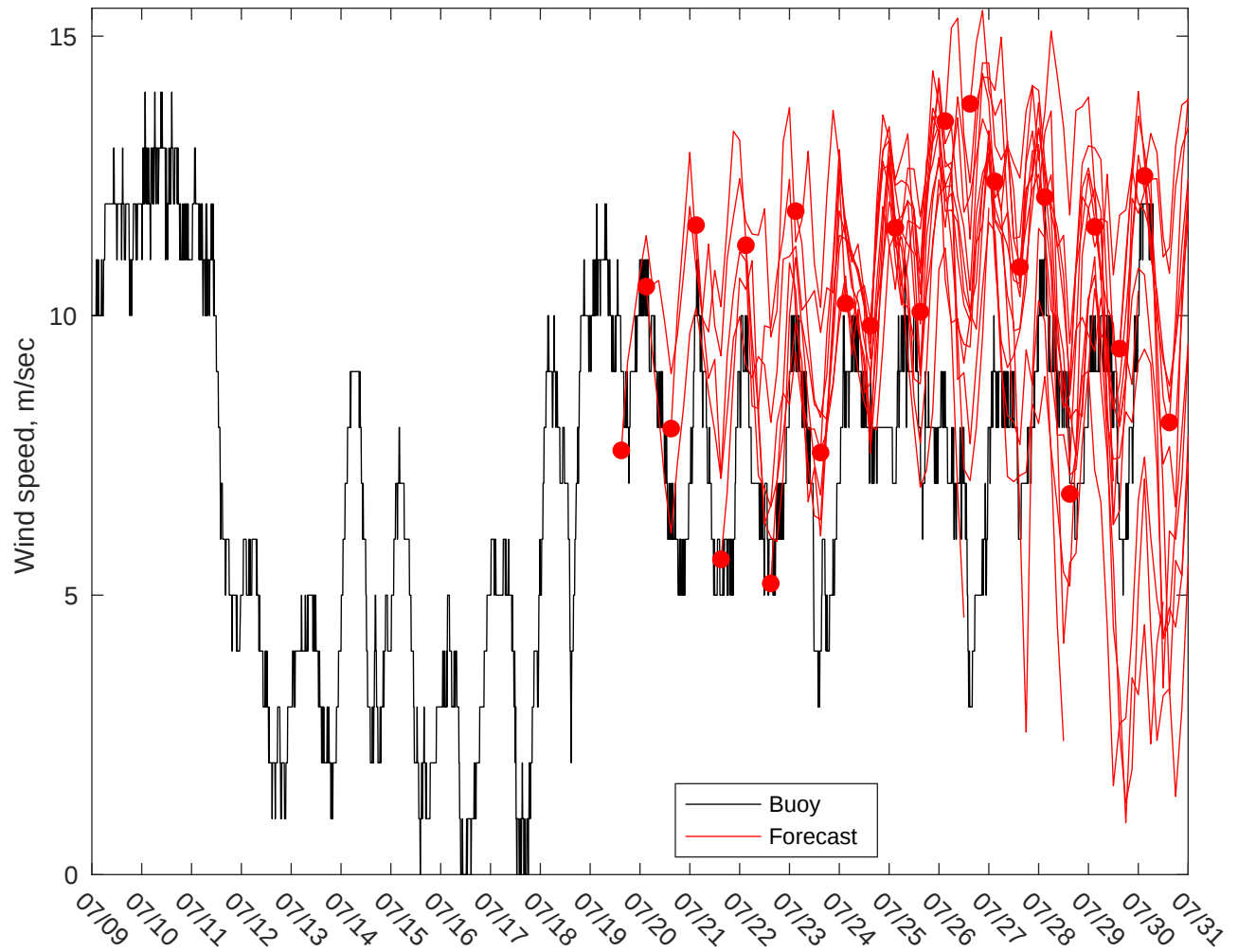
NDBC 46054 vs GFS Winds: 10 to 16 day forecast
