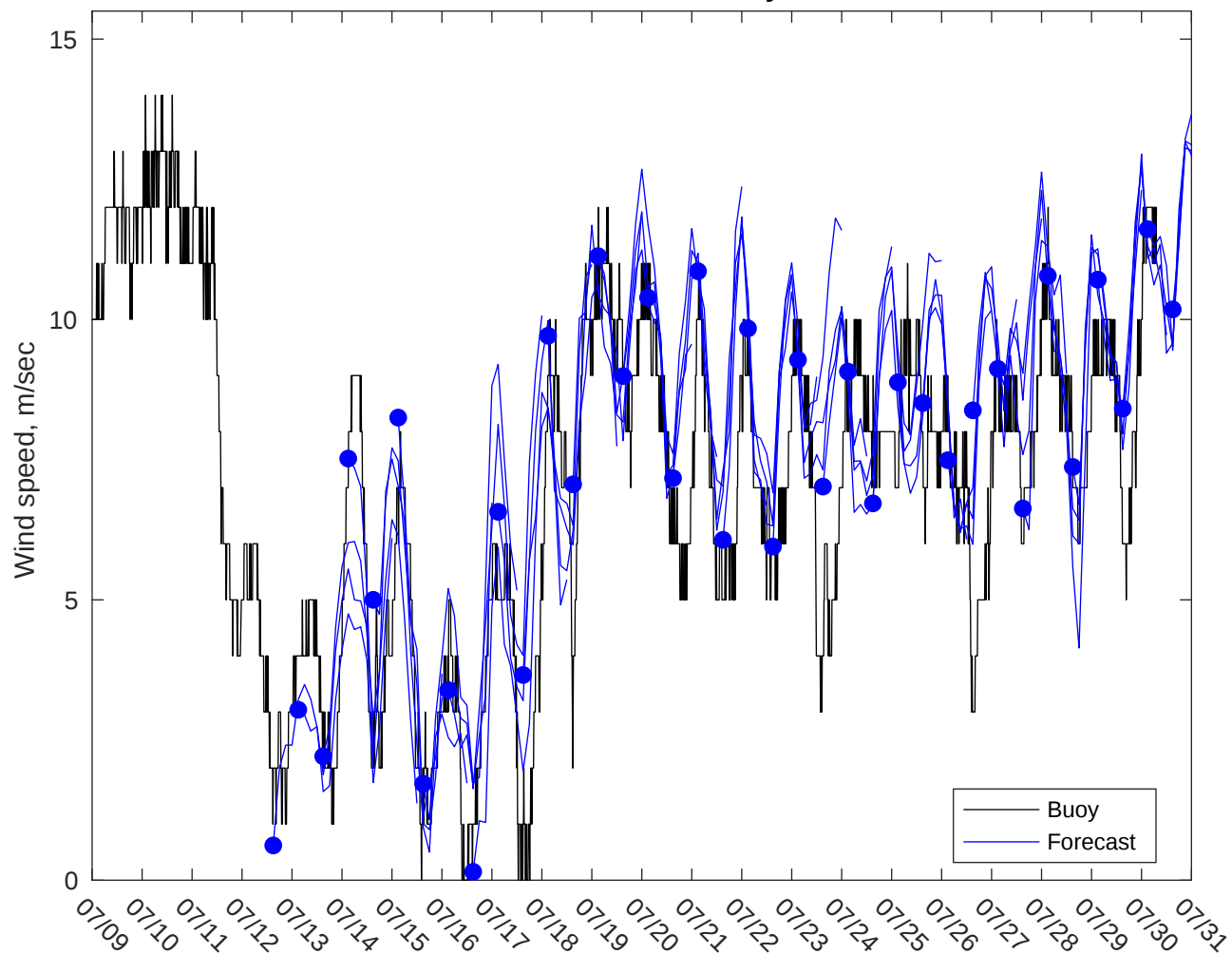
NDBC 46054 vs GFS Winds: 3 to 5 day forecast
