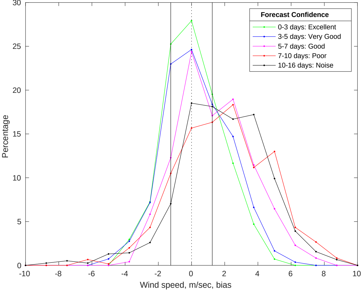
NDBC 46054 vs GFS Winds Bias Histogram: 30-Jul-2025
