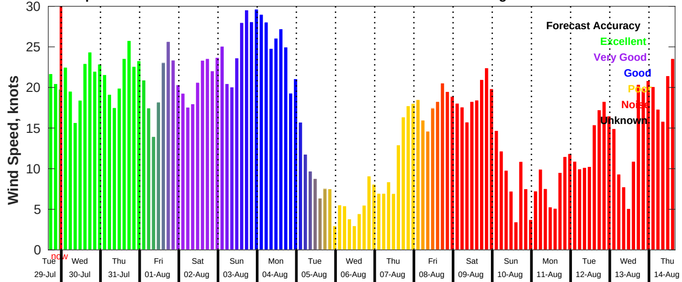
GFS Wind Speed Forecast for NDBC 46054 from 29-Jul-2025 16:00:00 to 14-Aug-2025 16:00:00
