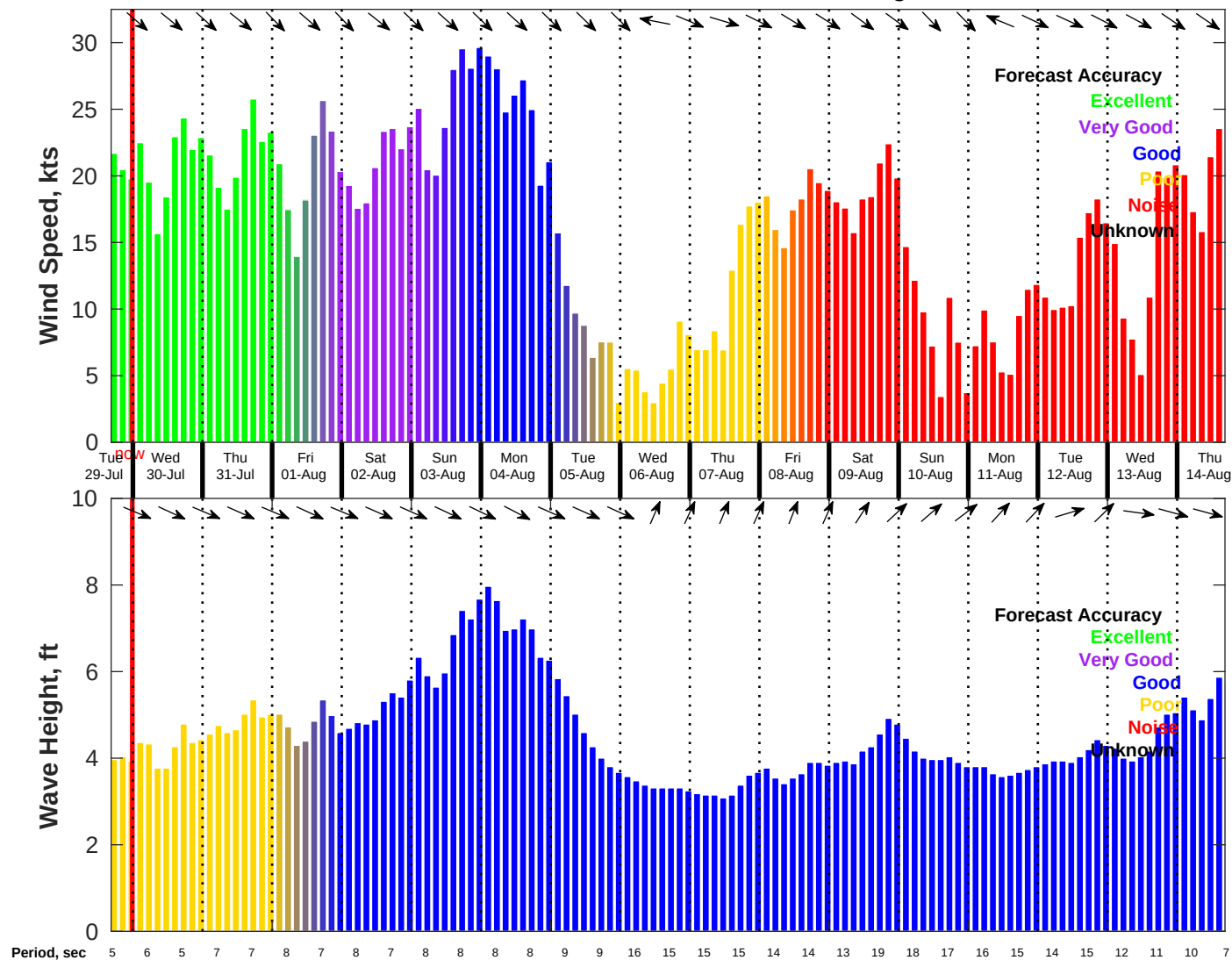
Wind & Wave Forecast for NDBC 46054 from 29-Jul-2025 16:00:00 to 14-Aug-2025 16:00:00
