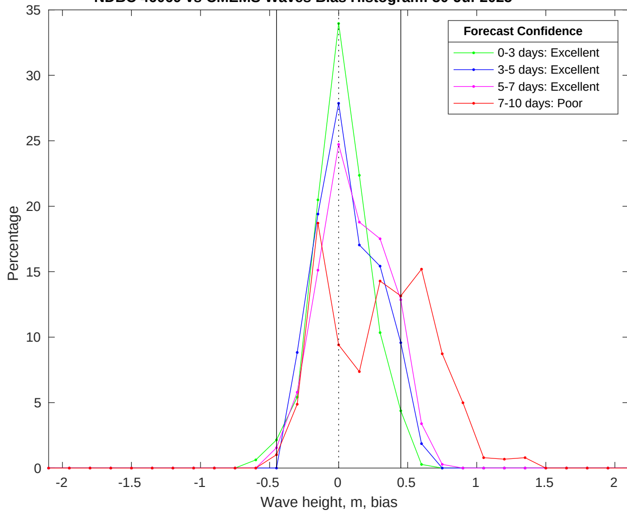
NDBC 46069 vs CMEMS Waves Bias Histogram: 30-Jul-2025
