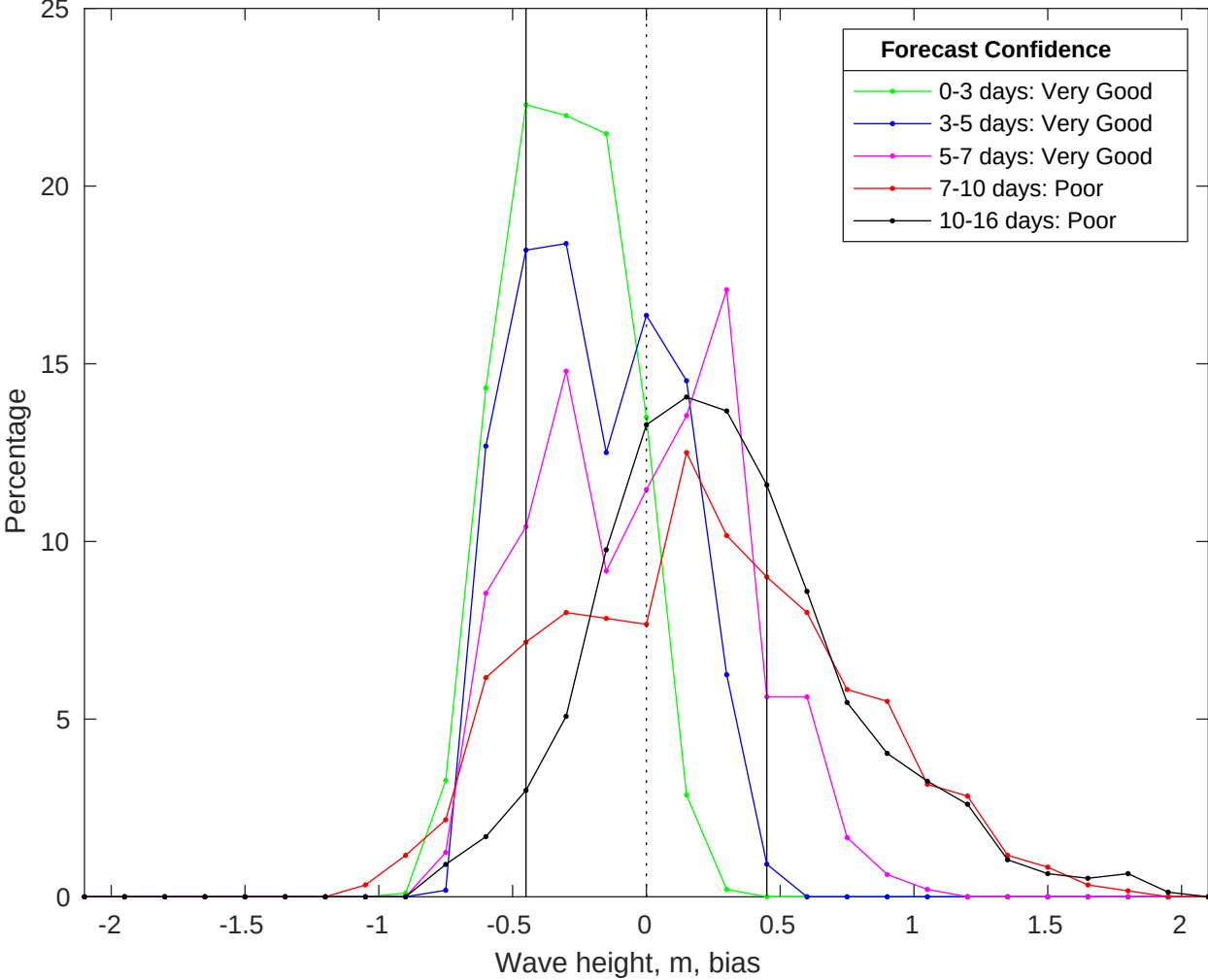
NDBC 46069 vs GFS Waves Bias Histogram: 30-Jul-2025
