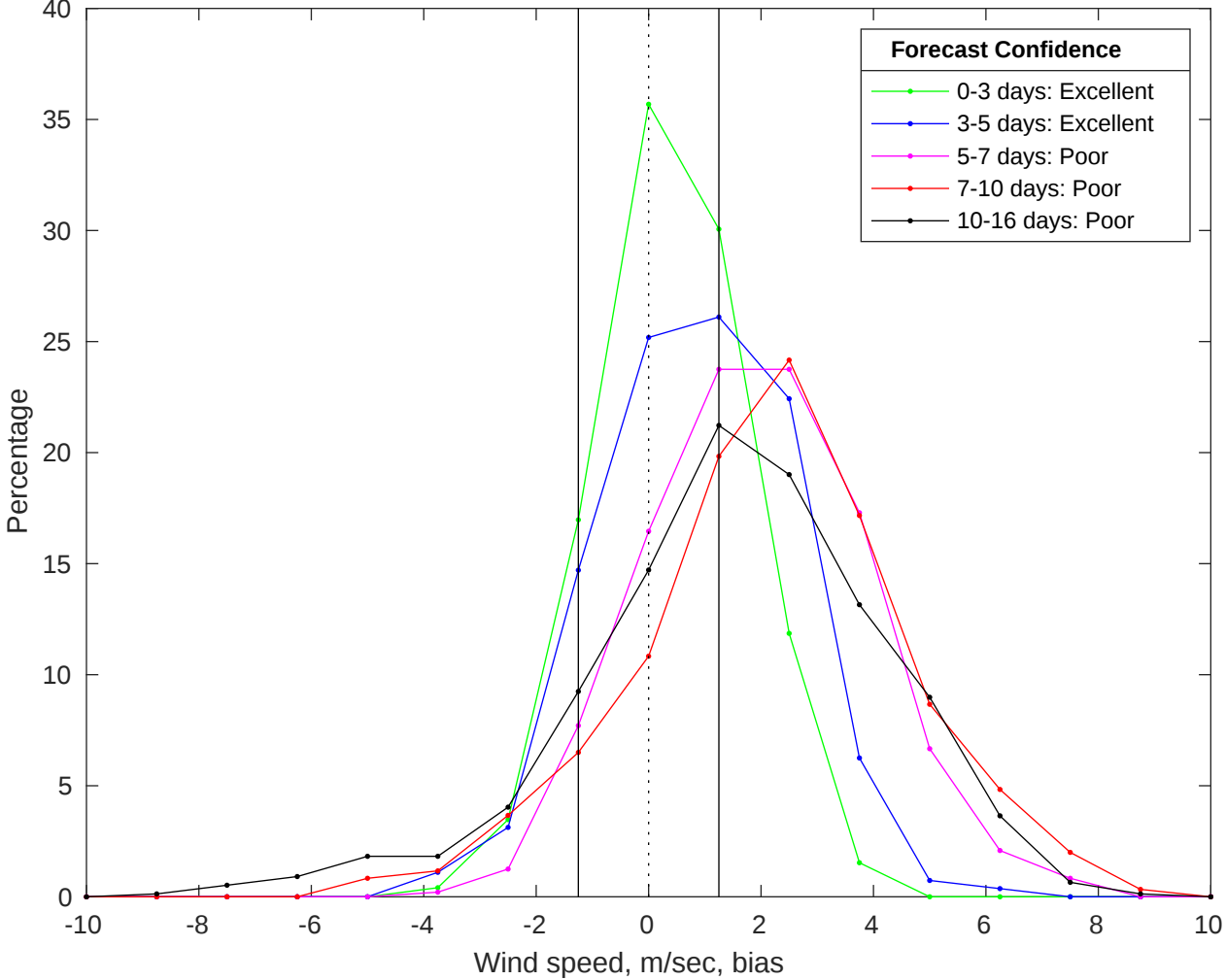
NDBC 46069 vs GFS Winds Bias Histogram: 30-Jul-2025
