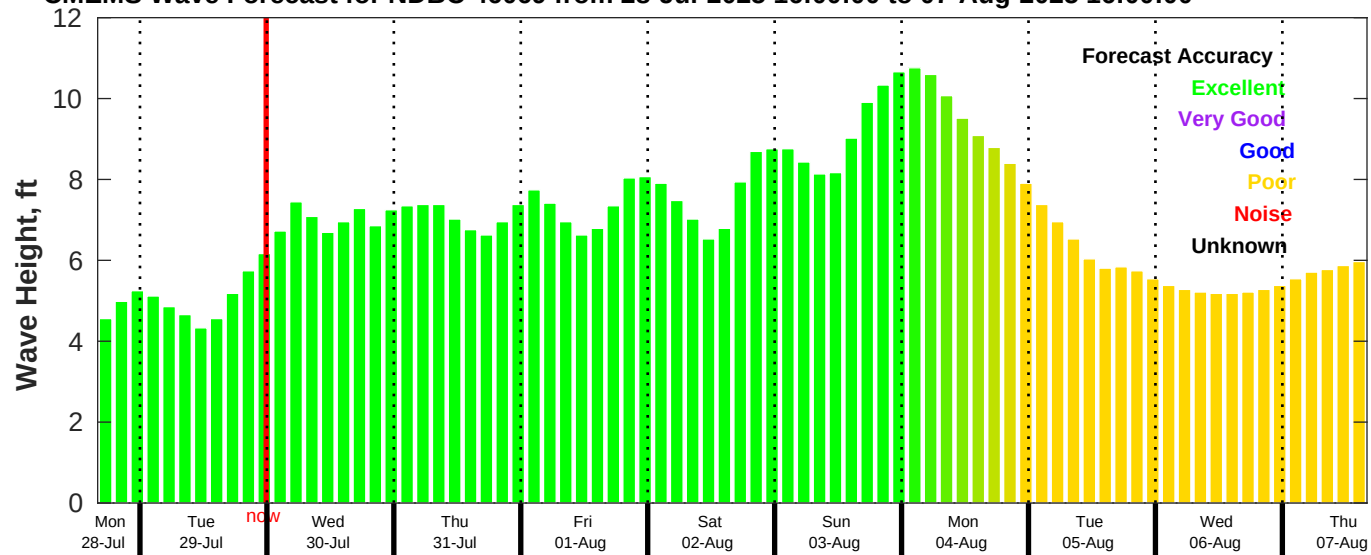
CMEMS Wave Forecast for NDBC 46069 from 28-Jul-2025 16:00:00 to 07-Aug-2025 16:00:00
