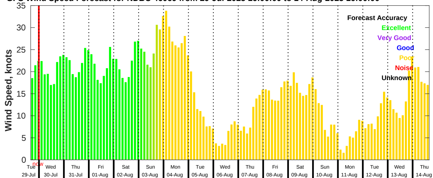
GFS Wind Speed Forecast for NDBC 46069 from 29-Jul-2025 16:00:00 to 14-Aug-2025 16:00:00
