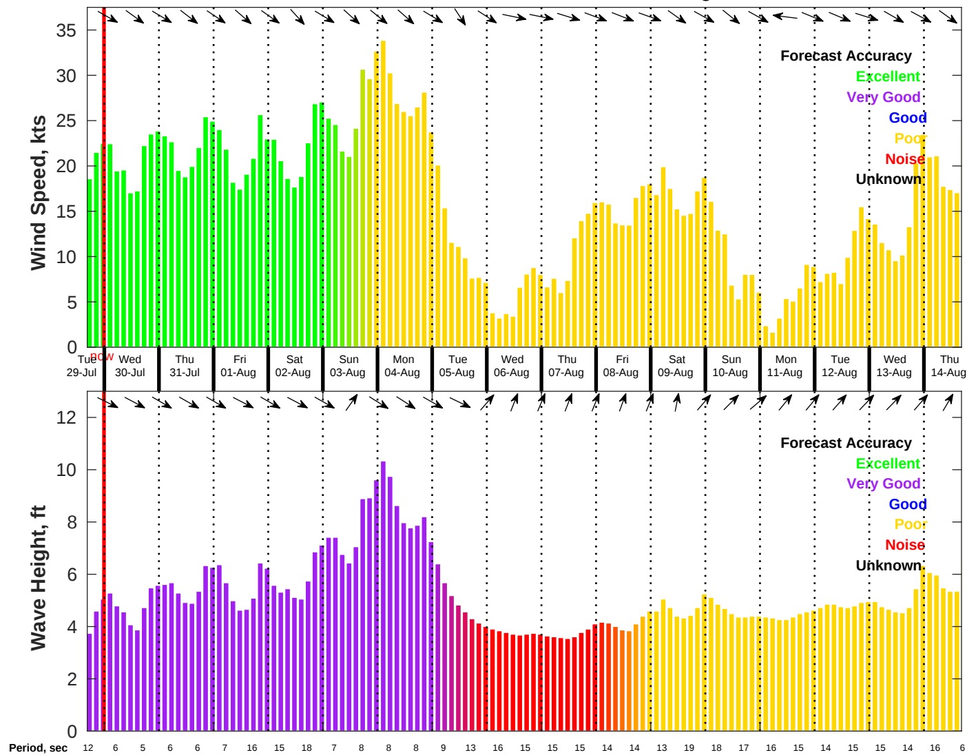
Wind & Wave Forecast for NDBC 46069 from 29-Jul-2025 16:00:00 to 14-Aug-2025 16:00:00
