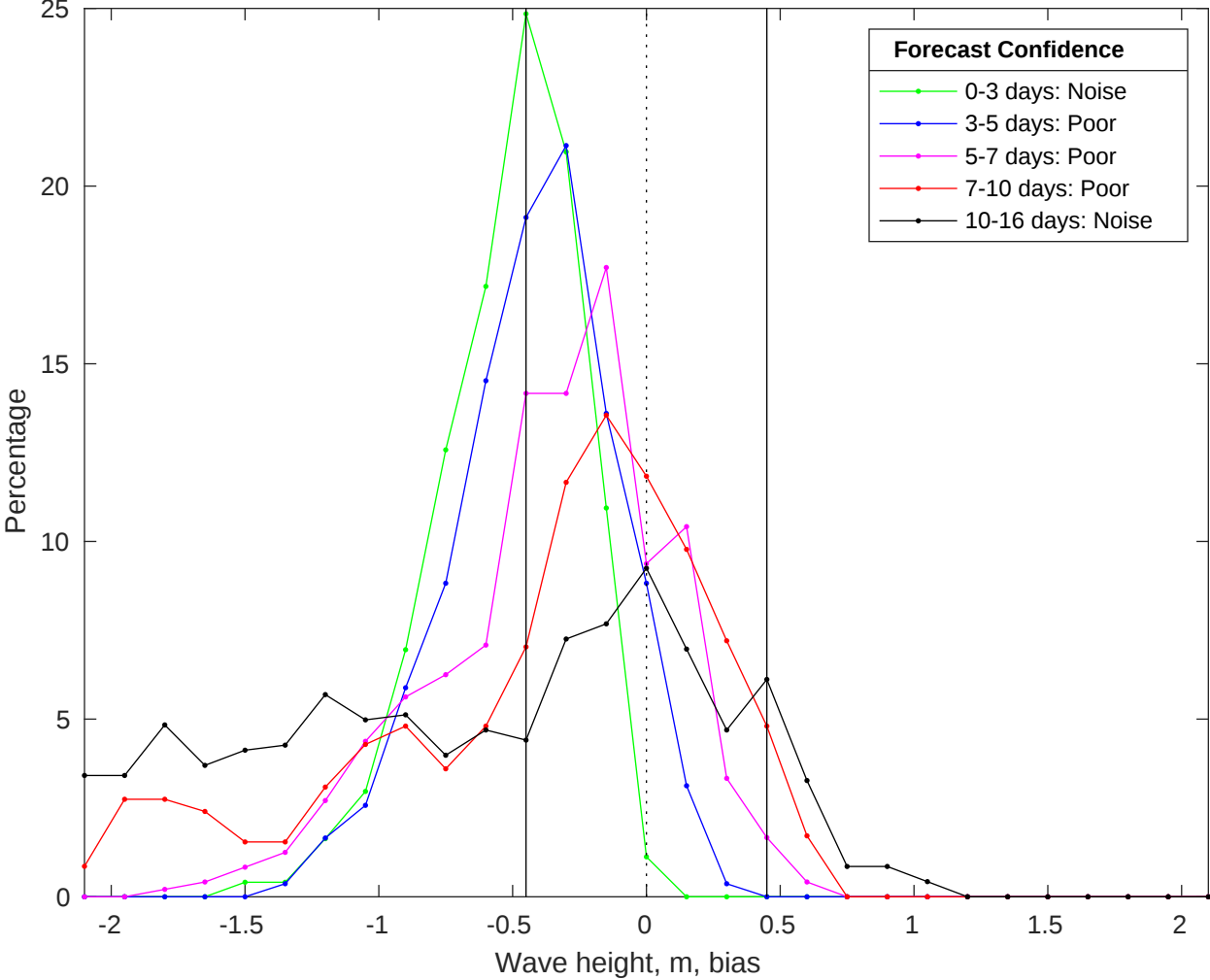
NDBC 51209 vs GFS Waves Bias Histogram: 30-Jul-2025
