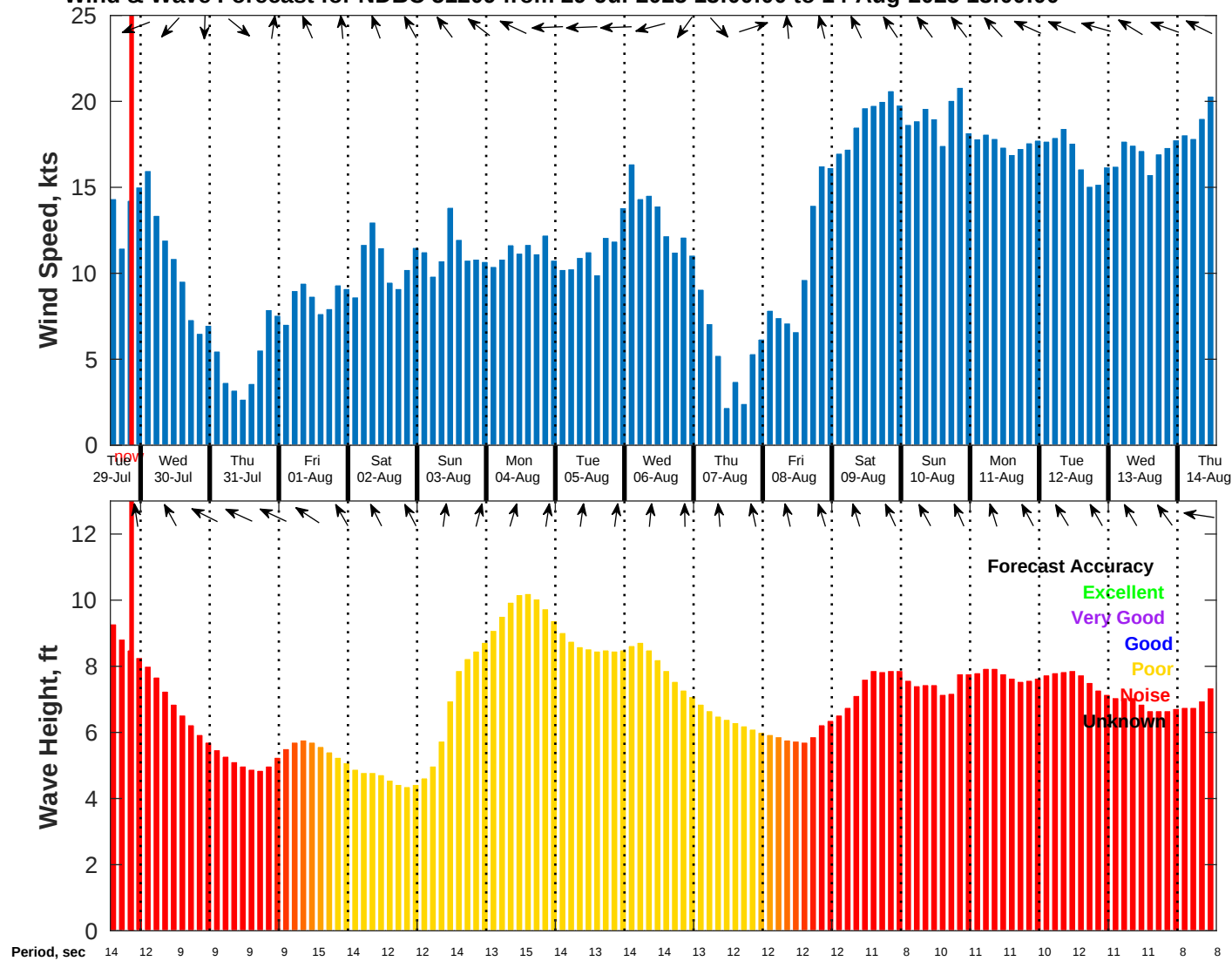
Wind & Wave Forecast for NDBC 51209 from 29-Jul-2025 13:00:00 to 14-Aug-2025 13:00:00
