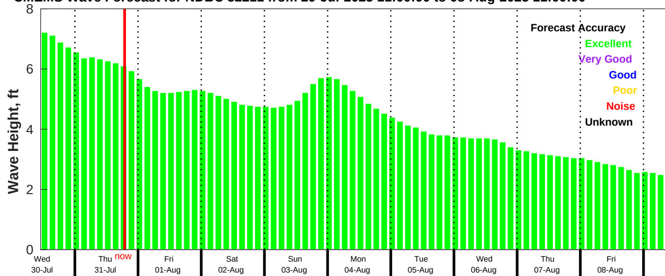
CMEMS Wave Forecast for NDBC 52211 from 29-Jul-2025 11:00:00 to 08-Aug-2025 11:00:00
