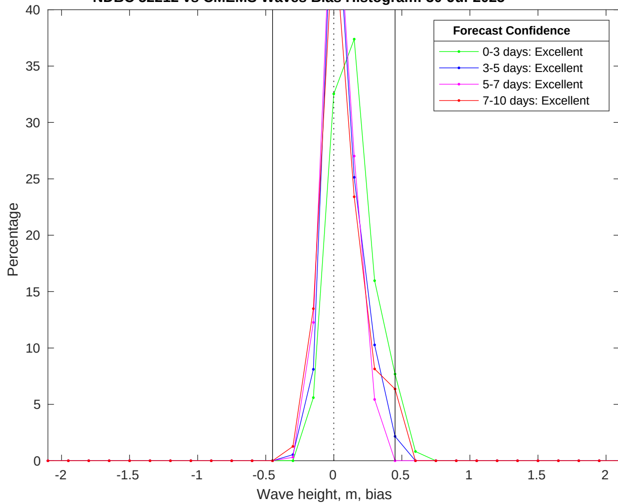
NDBC 52212 vs CMEMS Waves Bias Histogram: 30-Jul-2025
