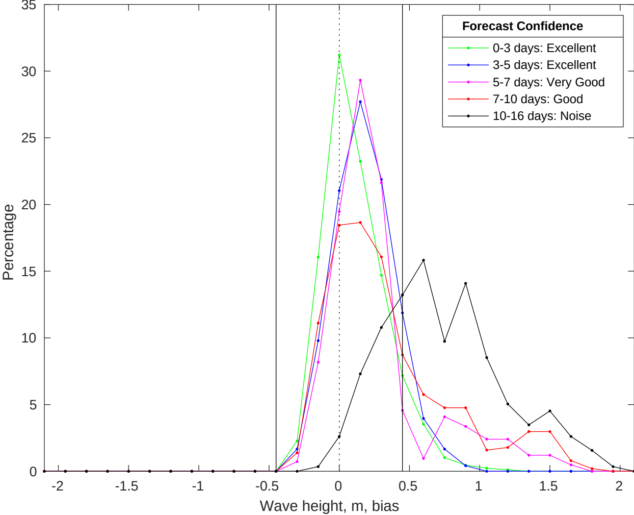
NDBC 52212 vs GFS Waves Bias Histogram: 30-Jul-2025
